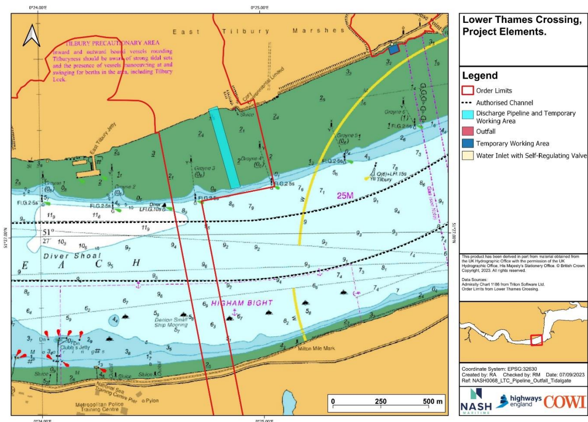
Plate 3.2 Discharge pipeline and outfall locations
